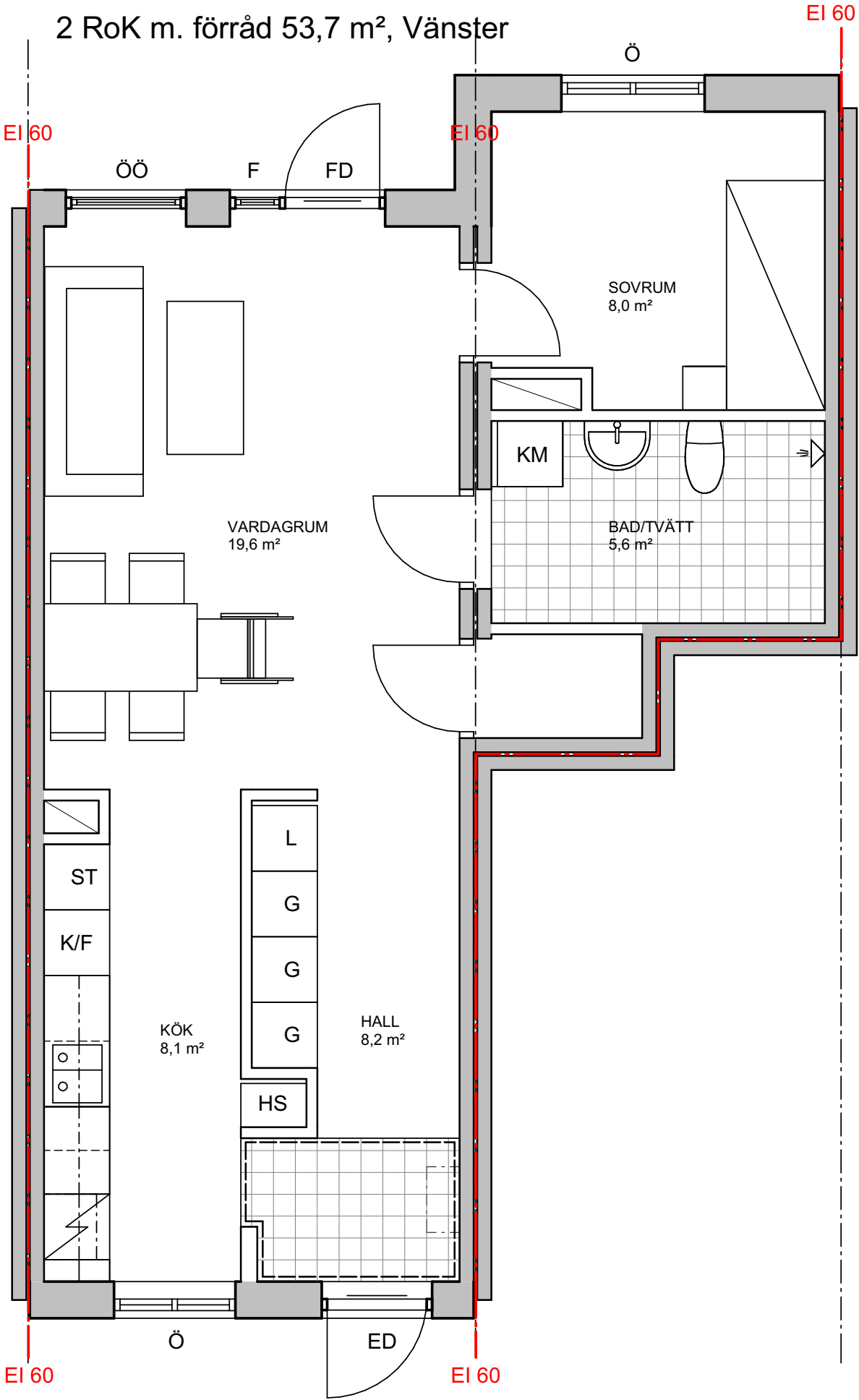
PLAN 2RoK
